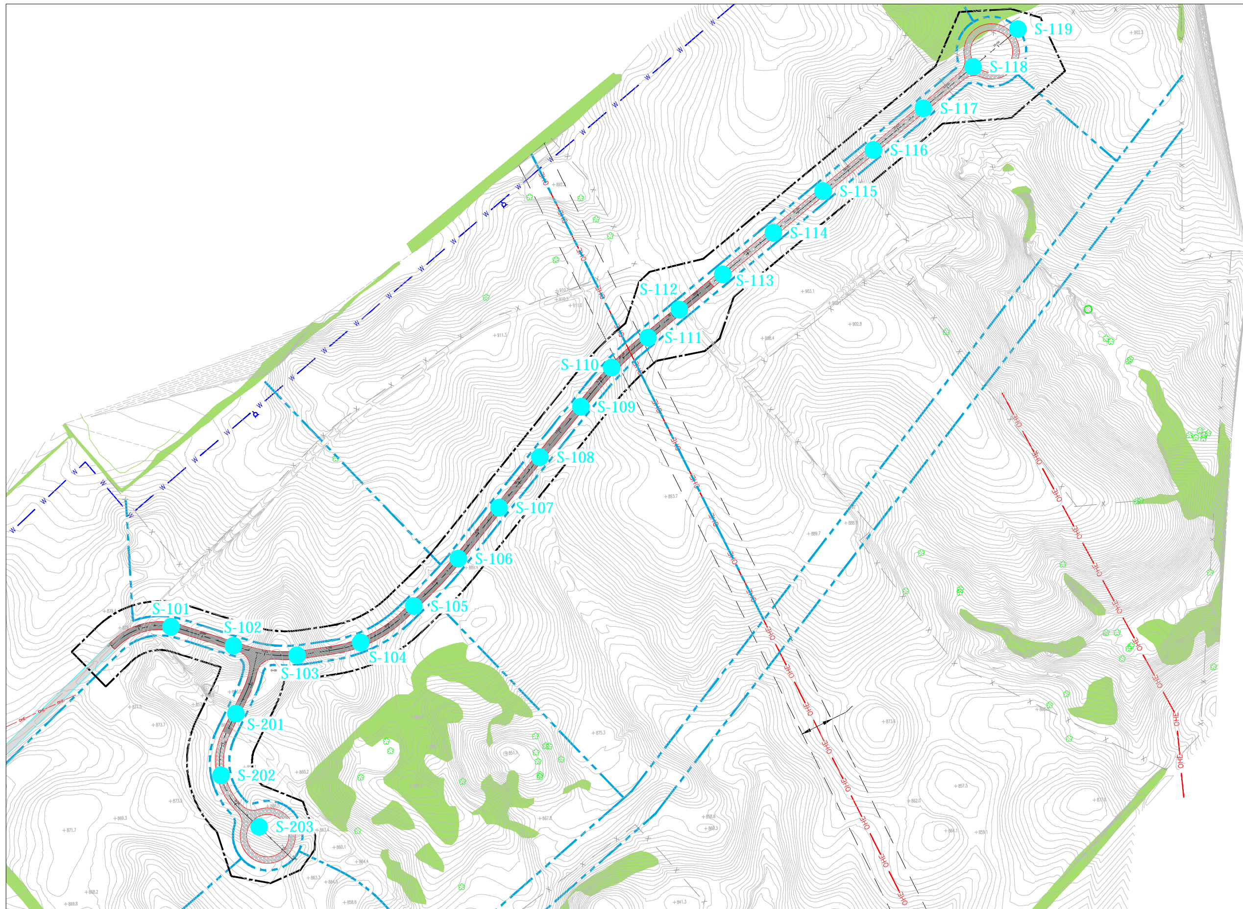
Boring Location Plan adapted from provided Realignment Plan dated August 8, 2020, with further adaptation by CSI personnel. Elevations were determined using Real Time Kinematic Differential GPS referencing the KYCORS network.
